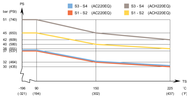
AC220EQ / ACH220EQ - PV code PED pressure/temperature graph
