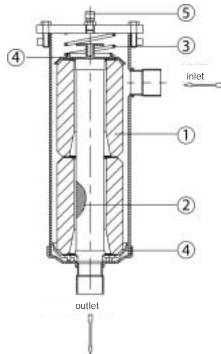
Sketch of filter with 2 blocks 1 - Block 2 - Mesh sieve serving as block support 3 - Spring 4 - Retainer cup 5 - Access fitting 1/4" SAE flare (to order separately)
